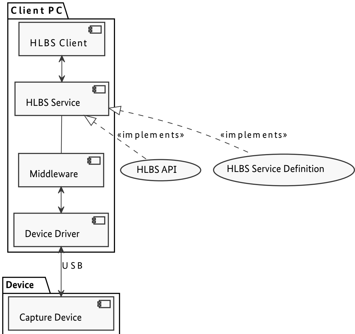
Figure 7.3. Architecture via USB
