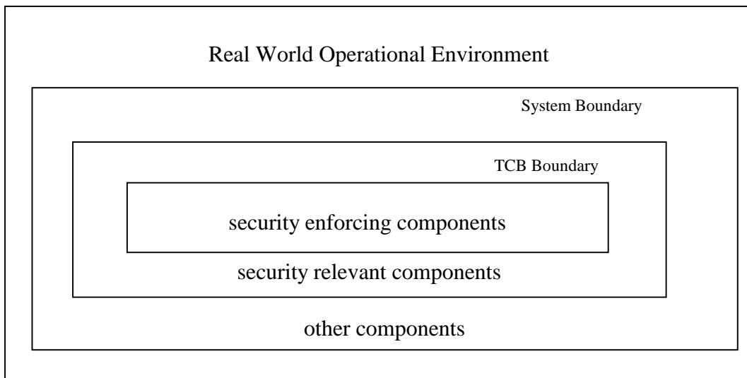
Fig. 1 IT System
