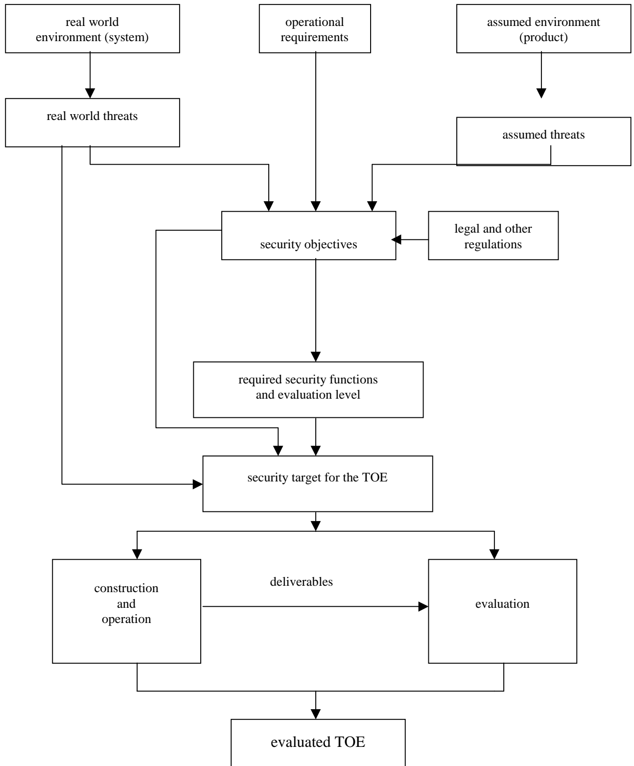
Fig. 3 Development and Evaluation Process
