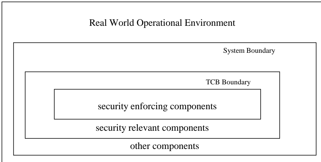
Fig. 1 IT System
