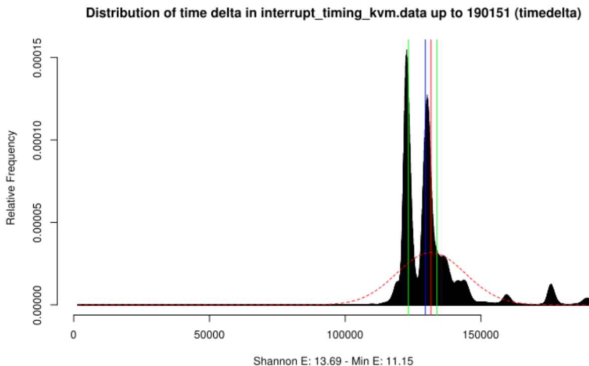
Figure 65: Histogram of High-Resolution Time Delta for Interrupts – KVM
