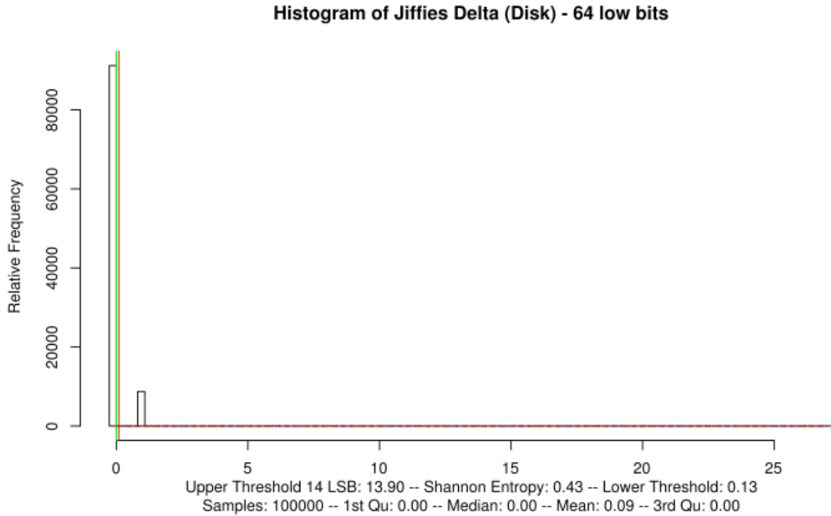
Figure 12: Histogram of Jiffies Delta for Block Device – KVM Without Buffer Cache
